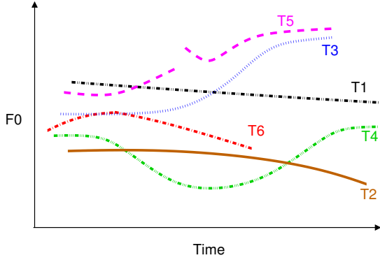
Figure 1: F0 contour of six different lexical tones of Vietnamese language: T1 (mid level), T2 (low falling), T3 (high rising), T4 (mid dipping-rising), T5 (high breaking-rising) and T6 (low falling constricted), adapted from [7].
