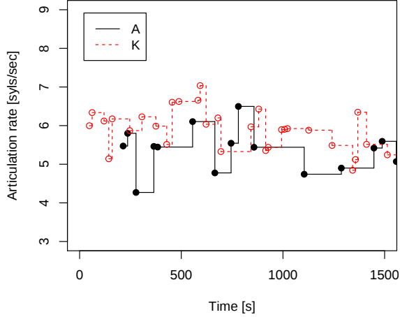
Figure 1: AR profiles for dialog A-K from the UM condition. Rates are assumed to be constant until the next long turn.
